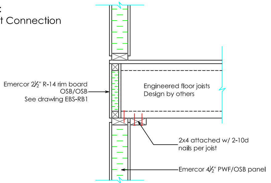
Alternate C: Foundation Panel to Joist Connection
