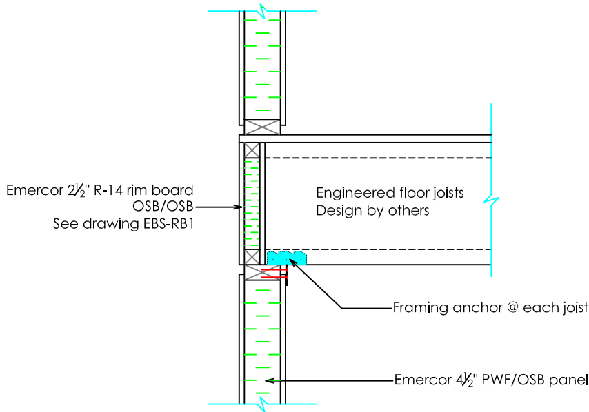
Alternate B: Foundation Panel to Joist Connection
