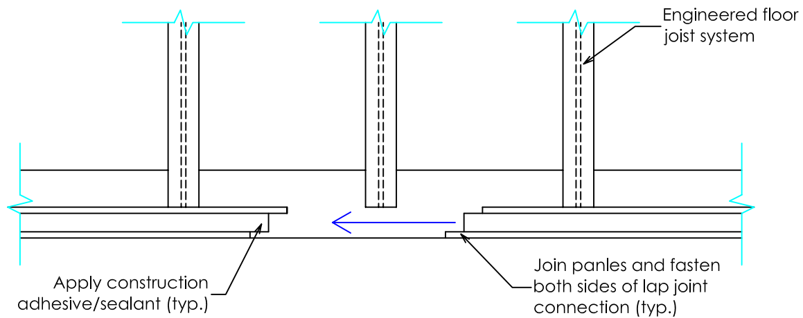
Top View
