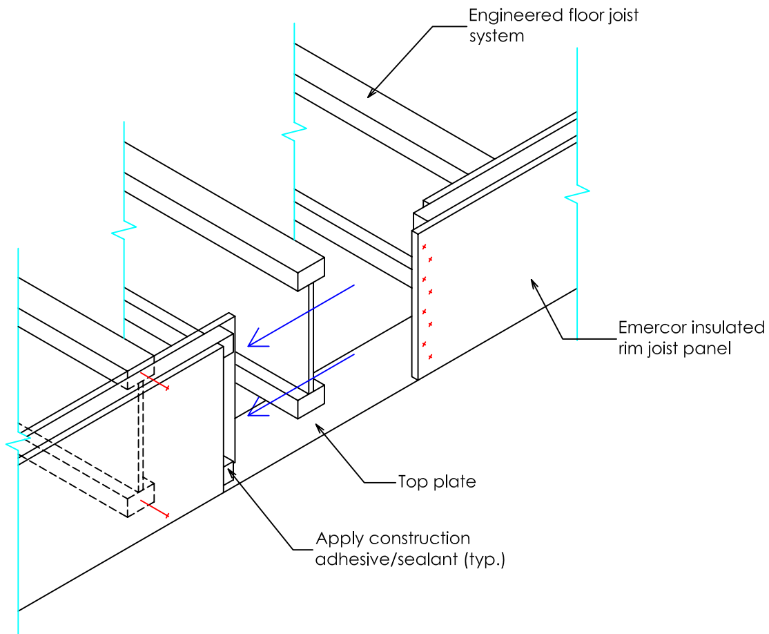
Isometric View
