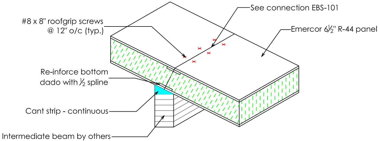
Intermediate Beam Connection
