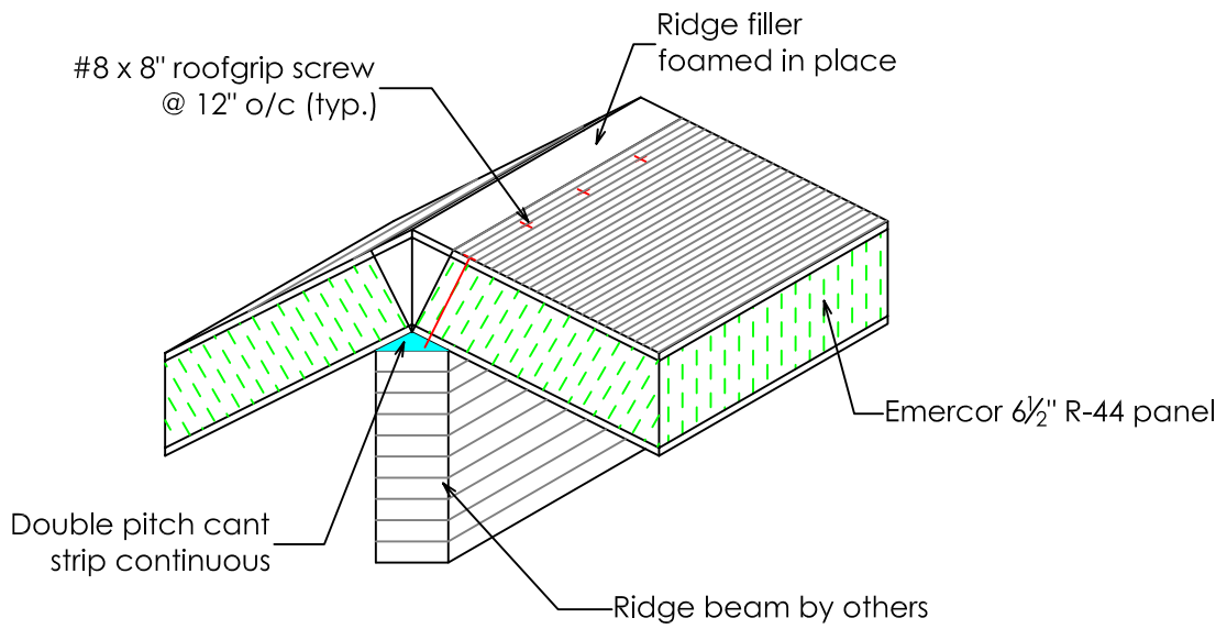
Ridge Beam Connection
